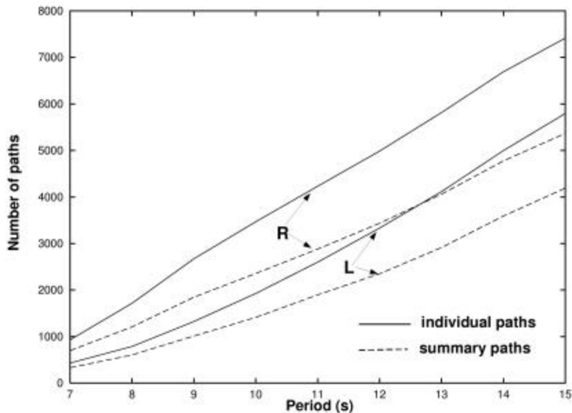
Figure 2. Number of individual and declustered measurements as a function of period for Rayleigh (R) and Love (L) waves.
