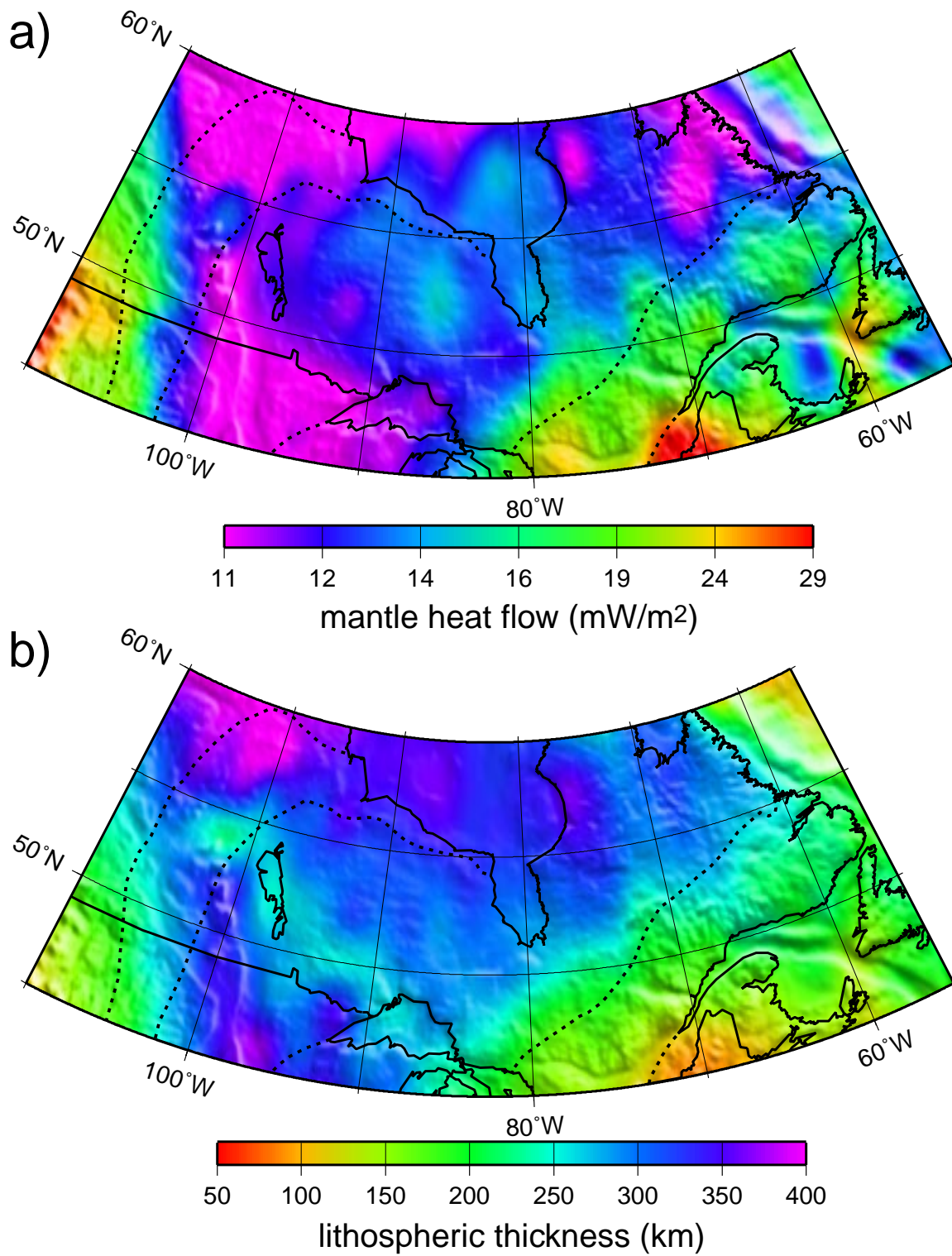
Figure 15. (a) The estimated mantle component of heat flow, Q_M . (b) The estimated lithospheric thickness, L . Dashed lines show boundaries of principal Precambrian provinces, adapted from Hoffman (1989).
