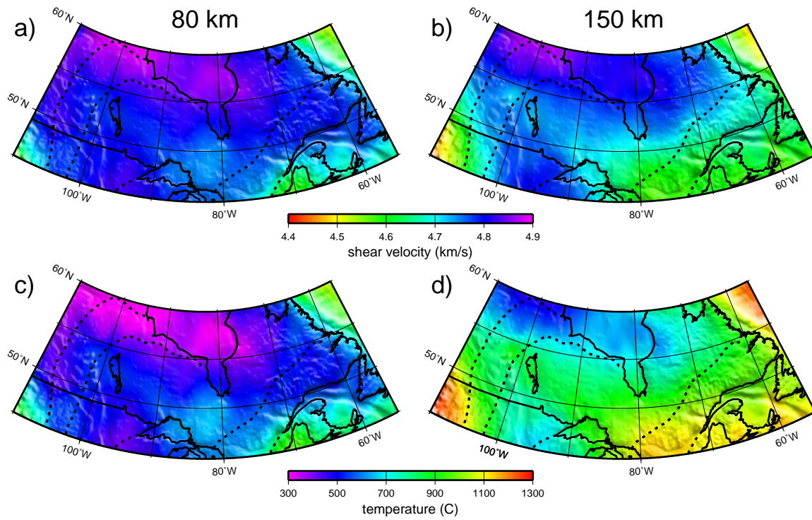
Figure 13. Horizontal slices of the seismic V_s = (V_{sh} + V_{sv})/2 model (a, b) and the temperature model (c, d) at depths of (a, c) 80 km and (b, d) 150 km. Dashed lines show boundaries of principal Precambrian provinces, adapted from Hoffman (1989).
