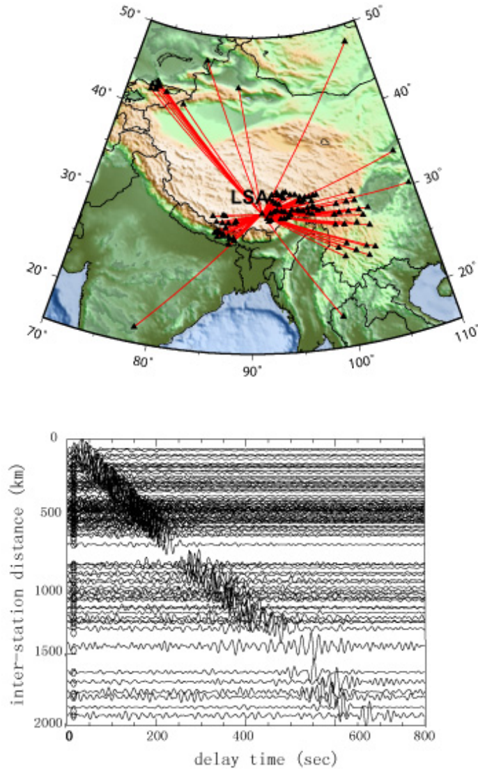
Figure 2: An example of a cross-correlation record-section with inter-station paths plotted in the top diagram for cross-correlation with \text{SNR} > 15 . The result is centered on station LSA (Lhasa, China), for the symmetric-signals, band-pass filtered from 10 - 30 sec.
