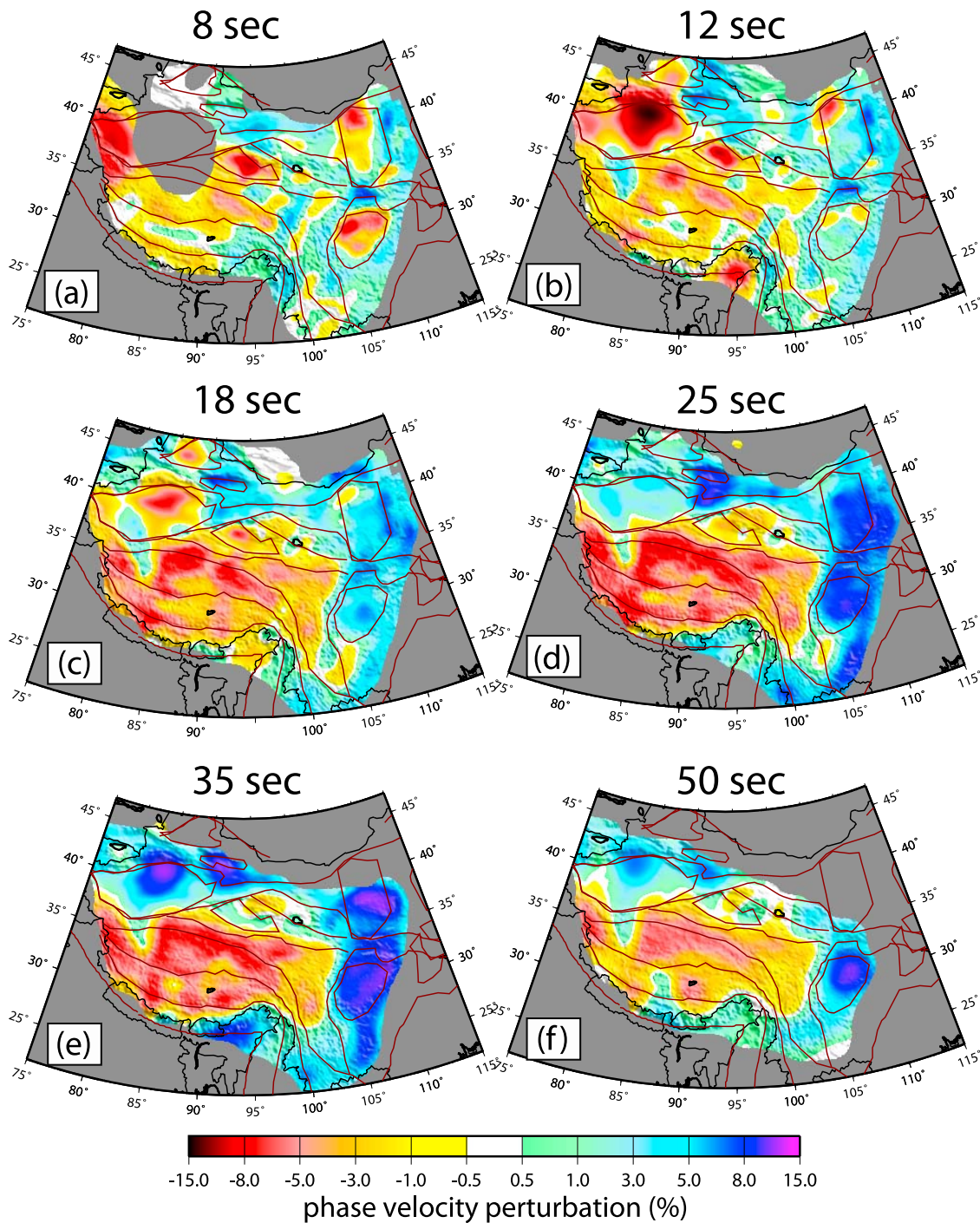
Figure 12. Phase velocity maps at periods of (a) 8, (b) 12, (c) 18, (d) 25, (e) 35, and (f) 50 s. Phase velocities are plotted as perturbations relative to the average value at each period. The maps truncate (reduce to gray shades) in regions where the resolution is worse than 400 km.
