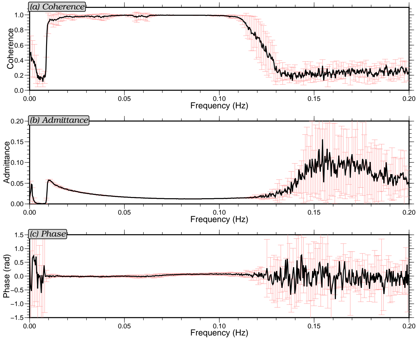
Figure 4. Example pressure-to-vertical compliance transfer functions for station J49A for the first nine days of March 2012. Similar to Fig. 3, black lines indicate the means of the transfer function characteristics over the nine days and the error bars are the standard deviations of the characteristic: (a) Coherence, (b) Admittance, and (c) Phase.
