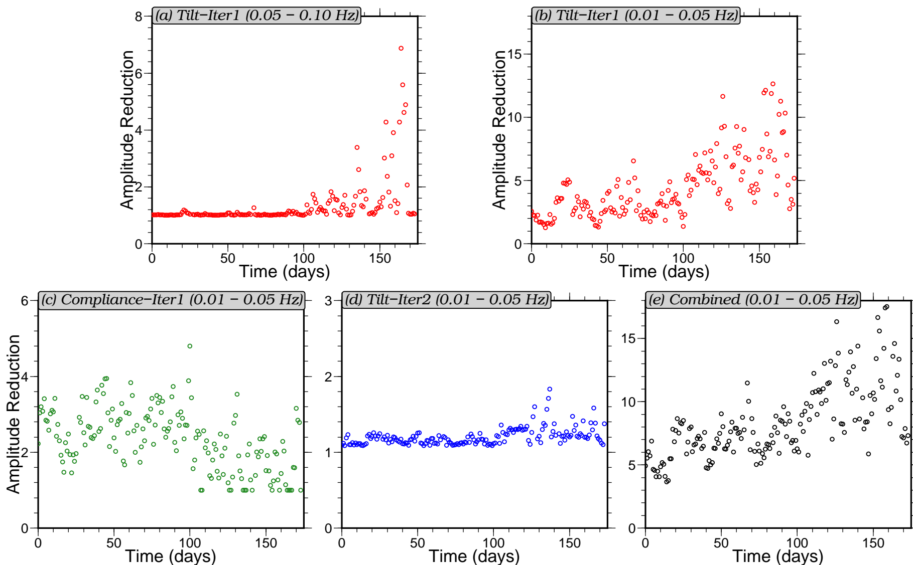
Figure 7. Daily averaged amplitude reduction (ratio) of the vertical component records for deep water station G03A. Each small circle in the diagrams indicates the daily averaged amplitude ratio of the record before and after the identified type of noise is removed. Horizontal axes present time in number of days where day zero is November 22, 2011, which is the first day with reasonable data for this station. (a) Amplitude reduction of removing tilt for the first iteration (10 - 20 sec period). (b) Similar to (a), but between 20 and 100 sec period. (c) Amplitude reduction of removing compliance for the first iteration (20 - 100 sec). (d) Amplitude reduction of removing tilt for the second iteration (20 - 100 sec). (e) Total amplitude reduction after two denoising iterations, combining the effects from (b), (c), and (d). A summary in three period bands of this total denoising statistic is presented for each station in Table 1.
