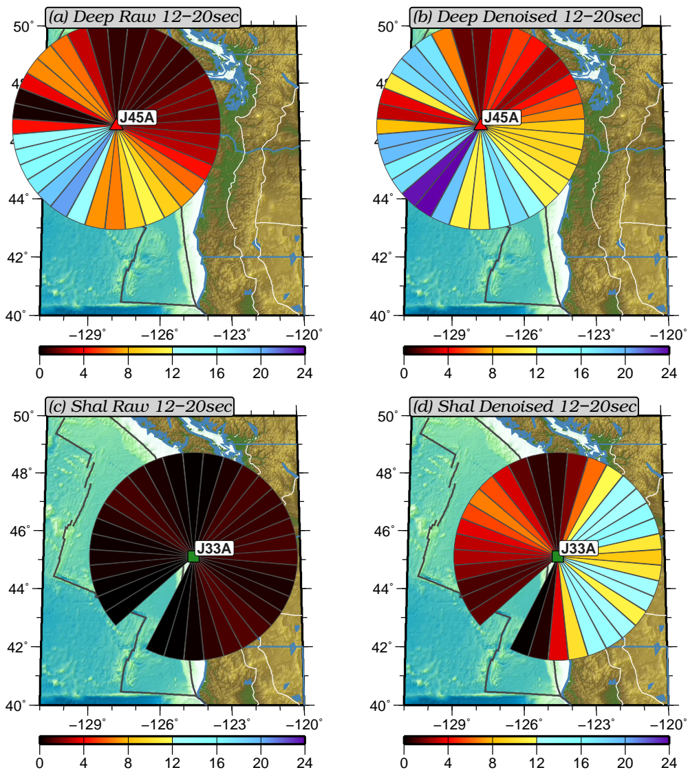
Figure 14. “Fan Diagrams” that summarize the azimuthal dependence of the amplitude of the primary microseism (12-20 sec). Cooler colors indicate strong signals pointing in the direction of propagation whereas warmer colors indicate weaker signal. (a) Deep water station J45A before the removal of tilt and compliance noise. (b) Same as (a), but after the removal of tilt and compliance noise. (c) Shallow water station J33A before the removal of tilt and compliance noise. (d) Same as (c), but after the removal of tilt and compliance noise.
