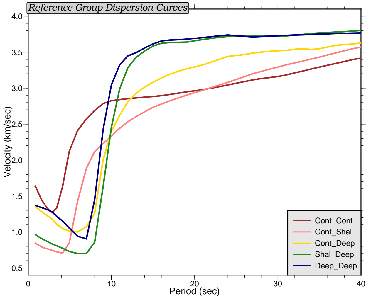
34 Figure 11. Reference group velocity curves, which are averages of measured curves between 35 stations located in different regions: continent-continent, continent-shallow ocean, continent-deep 36 ocean, shallow ocean-deep ocean, and deep ocean-deep ocean. 37 38
